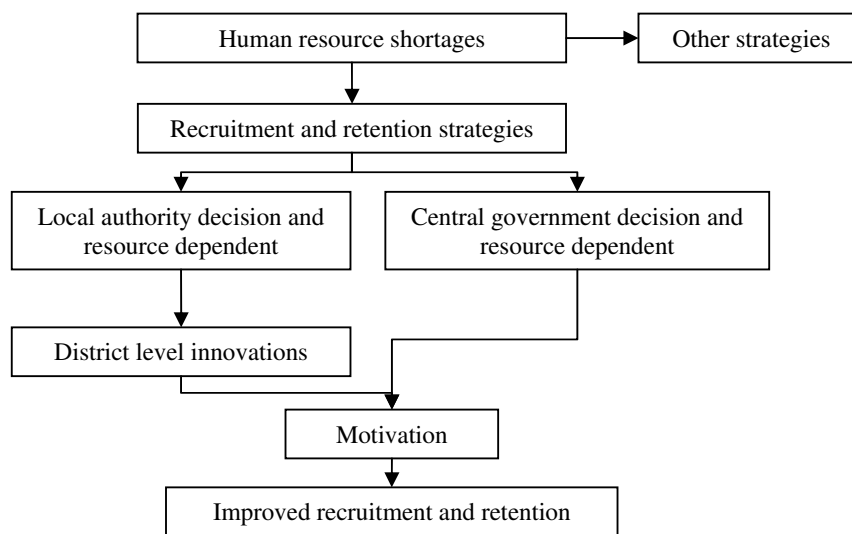
Figure 13.2 Analytical framework
